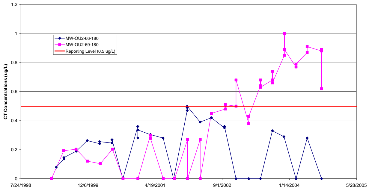
Figure 7. Carbon Tetrachloride Concentrations, Southern Lower 180-Foot Aquifer Plume
