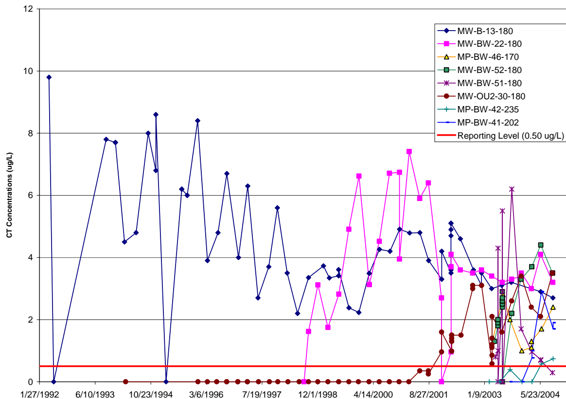
Figure 5. Carbon Tetrachloride Concentrations, Eastern Upper 180-Foot Aquifer Plume
